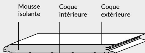
Panneaux double coque (figure 2)
